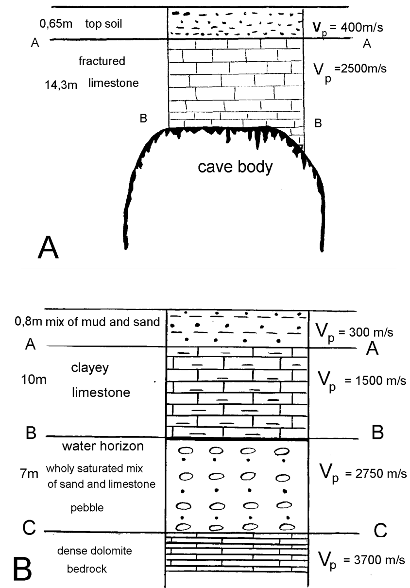
Fig.2 Samples of investigated vertical cross-sections (not to scale) of the subsurface at the experimental site: A - with a cave dome, B - with a water horizon.
