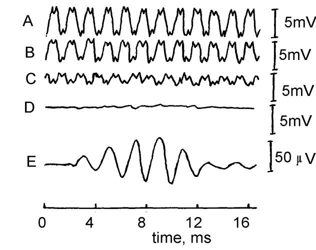
Fig.1 Noise reduction in the electric data. Trace A - electric signal recorded by antennas; traces B and C - remote noise records; trace D - result of linear combination of traces B and C subtracting from the trace A; trace E - result of trace D magnified by 100 and of the use of low pass filtering.
